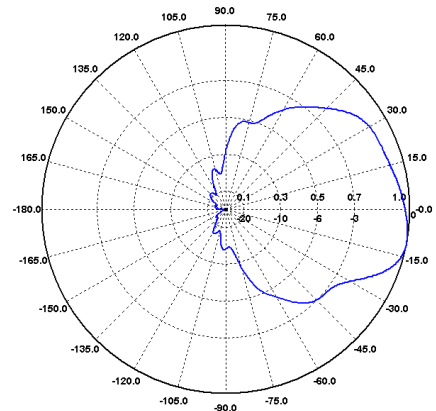
H-Ebene / H-Plane 1200 MHz
