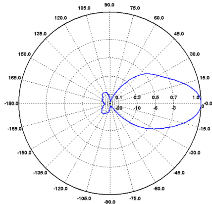
E-Ebene / E-Plane 900 MHz
