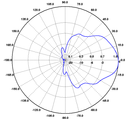
H-Ebene / H-Plane 1400 MHz
