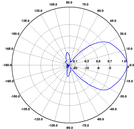
E-Ebene / E-Plane 1400 MHz
