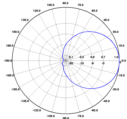
H-Ebene / H-Plane 500 MHz
