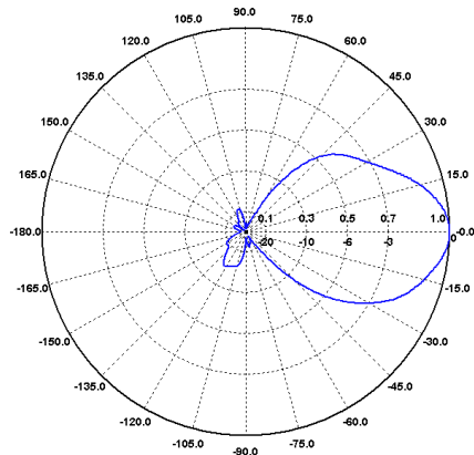
E-Ebene / E-Plane 1200 MHz
