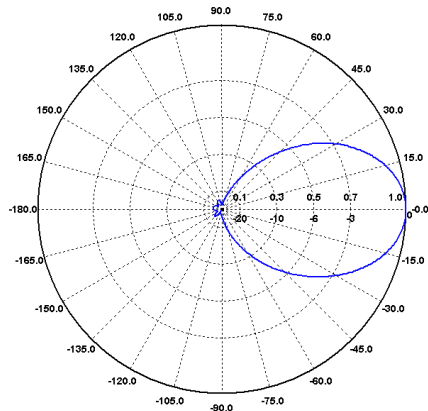
E-Ebene / E-Plane 500 MHz
