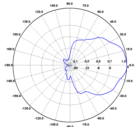
H-Ebene / H-Plane 1600 MHz
