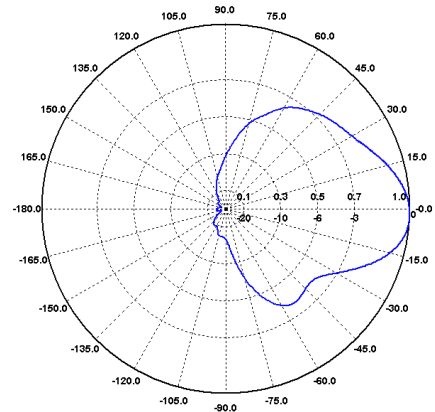
H-Ebene / H-Plane 900 MHz
