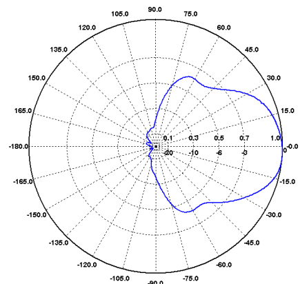
H-Ebene / H-Plane 1000 MHz
